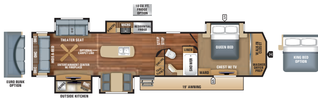
NORTH POINT | 361RSFS Ext. Lgth: 43' 7" Ext. Ht: 158" Unloaded Wt. (lbs): 13,590 Sleeps: 4
